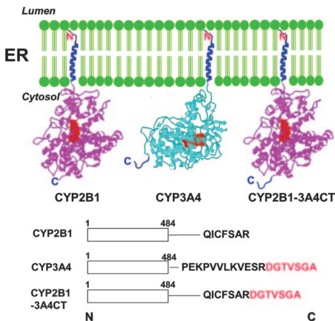
Fig. 5. The chimeric CYP2B1-3A4CT construct. The N-terminally anchored P450s 2B1, 3A4, and 2B1-3A4CT in the ER bilayer are schematically depicted (top). N and C refer to the P450 extreme N and C termini, respectively. The C-terminal amino acid sequence of each P450 beyond residue 484 is shown in its entirety (bottom). The chimeric CYP2B1-3A4CT protein consists of the extreme CYP3A4 C-terminal D 497 GTVSGA 503 peptide grafted onto the CYP2B1 C terminus. For details, see Materials and Methods .
