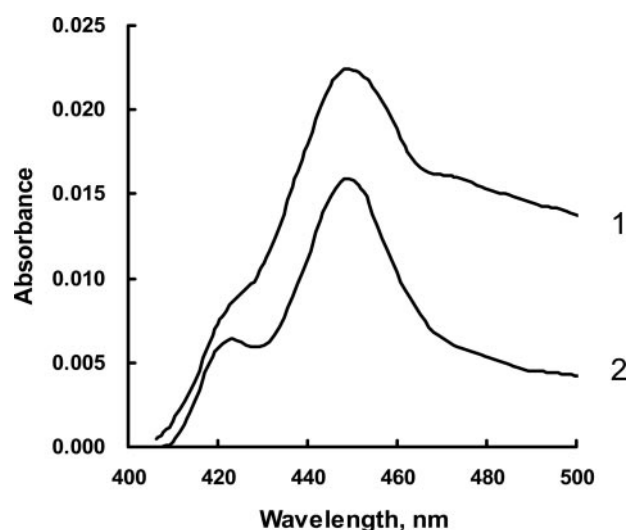
Fig. 9. Spectrally detected microsomal P450 content. Yeast strain RHY718 ( wt , HRD ) transformed with either expression plasmid (1) pYcDE/2B1 (CYP2B1) or (2) pYcDE/2B1-3A4CT (CYP2B1-3A4CT) was grown at 30°C in SD with appropriate supplements. Cells were harvested during logarithmic growth phase (early stage), and the reduced CO-difference spectra of yeast microsomal CYP2B1 and CYP2B1-3A4CT preparations (2 mg of protein/ml) were determined as described previously (Murray and Correia, 2001).
